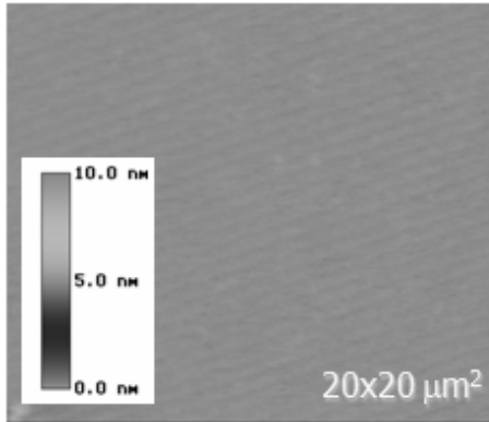
Figure 2. An AFM image of a c-plane wafer after chemical mechanical polishing. The RMS roughness is 0.063nm.
