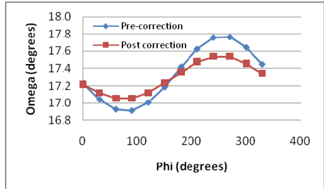
Figure 1: Off-cut calculation using XRD measurement
