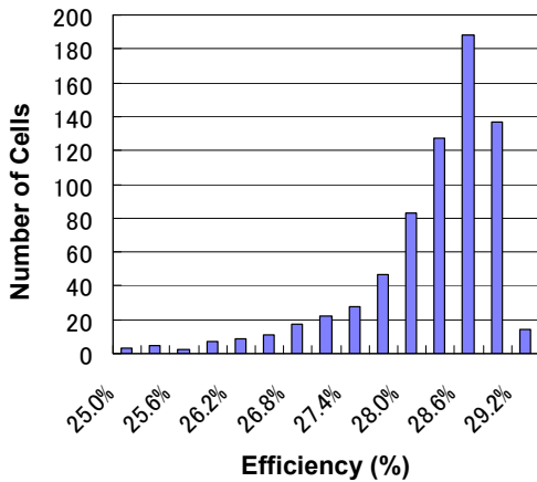
Figure 3: Distribution of efficiency in production of space solar cells, as an example for JAXA program.
