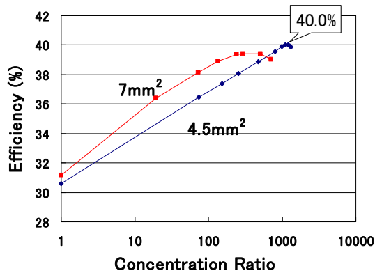
Figure 7: Efficiency as a function of concentration ratio for the cells with different size.
