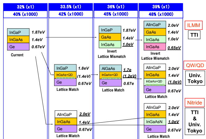
Figure 8: High efficiency approach in NEDO innovative solar cell development project
