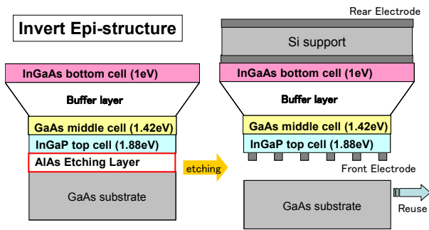
Figure 9: Cell fabrication process to realize high efficiency InGaP/GaAs/InGaAs(1eV) triple-junction cell.
