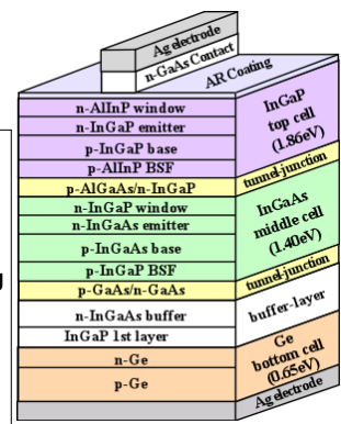
Figure 2: Schematic of the main stream triple junction structure and key techniques for improving efficiency
