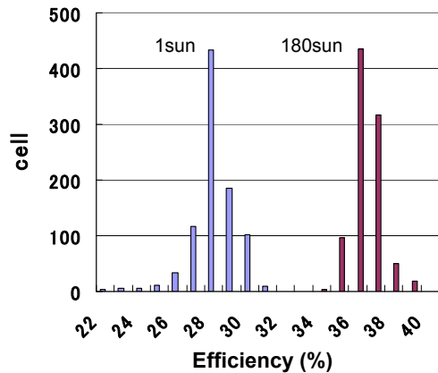
Figure 4: Distribution of efficiency in production of concentrator solar cells for CPV system in-house..
