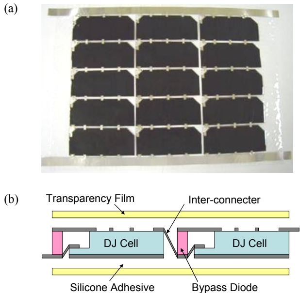
Figure 5: (a) Photograph of space solar sheet and (b) schematic cross section view.
