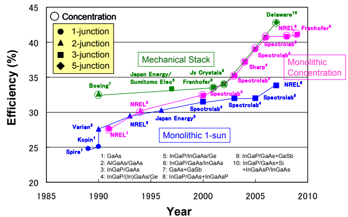
Figure 1: Progress in world record conversion efficiency of compound solar cells
