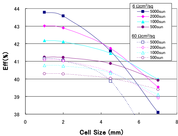
Figure 6: Increase in efficiency by reducing cell size, as a dependence of sheet resistance. (Calculation)
