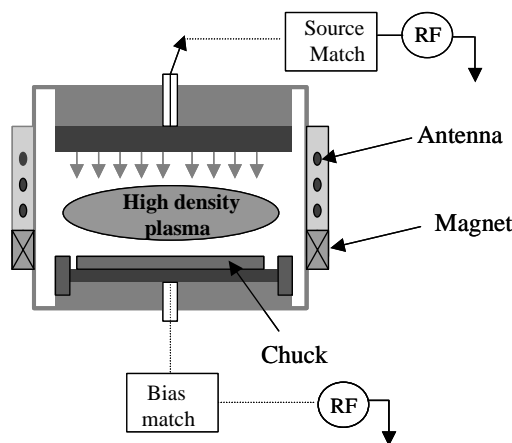
Figure 1. Configuration of an HD-ICP-CVD system using \text{SiH}_4/\text{N}_2 for silicon nitride passivation on 0.15\mu\text{m} GaAs PHEMTs.
