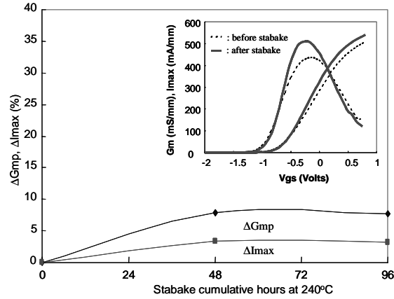
Figure 4. Thermal stability examination of HD-ICP-CVD passivated GaAs PHEMTs (Insert: recovery of characteristics of G_m and I_{ds} versus V_{gs} after stabake at 240^\circ\text{C} for 48 hours).
