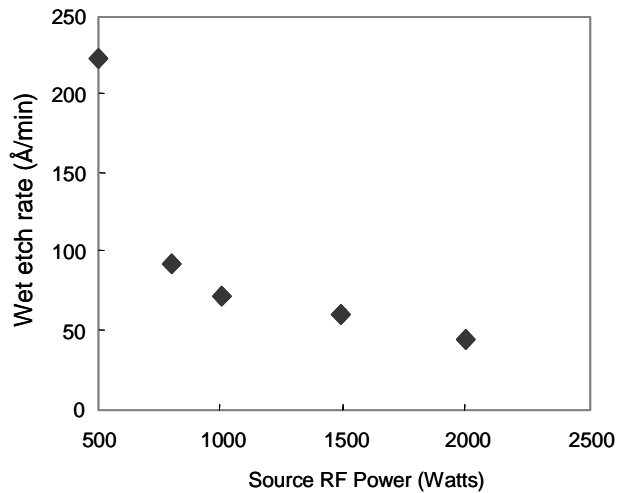
Figure 2. Wet etch rate of HD-ICP-CVD's nitrides as a function of ICP source power at a deposition temperature of 170^\circ\text{C} .
